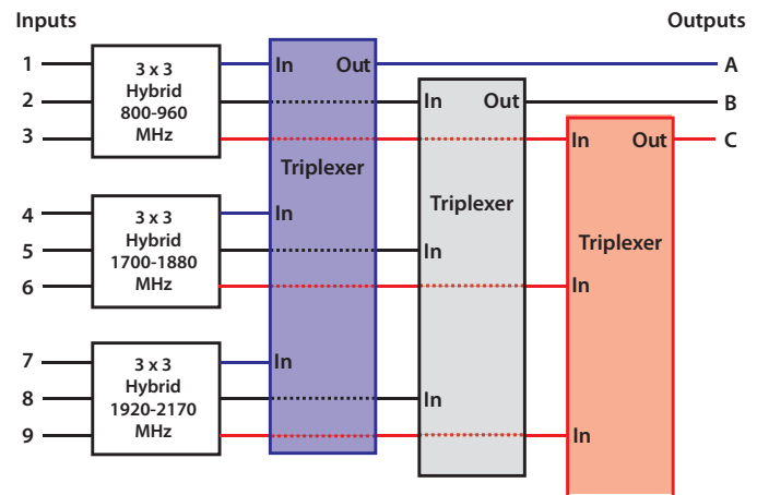
Fig 1: ‘Lossless’ combining of 9 inputs to 3 distributed antenna feeds, as might be used in an in-building DAS system.
