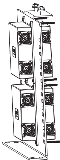
SPLITTER MOUNTING 1-4 SPLITTERS
